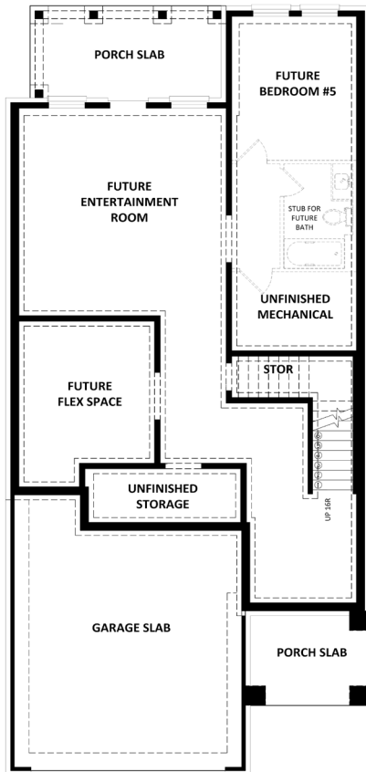
Opt. Basement Floor Plan
