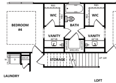
Second Floor Plan W/Opt. Third Floor
