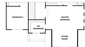
Second Floor Plan w/ Opt. 2nd Closet
