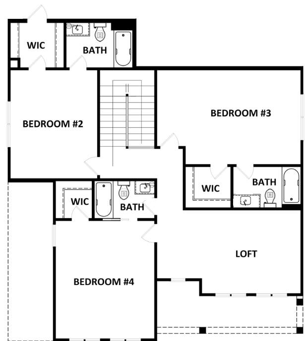
Second Floor Plan "C"
