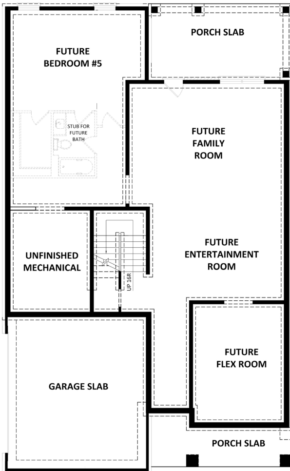
Opt. Basement Floor Plan
