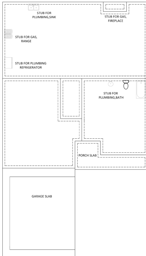
Slab Floor Plan
