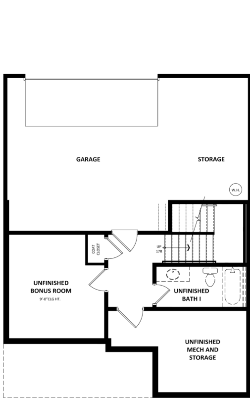
Basement Floor
